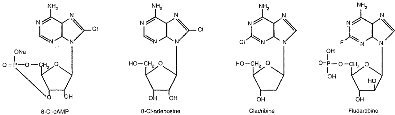
Figure 5 Structures of 8-Cl-cAMP, 8-Cl-adenosine, cladribine (2-chloro-deoxy-adenosine) and fludarabine (2-fluoro-adenine arabinoside-5'-phosphate)
